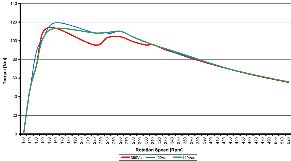
Torque Curve
