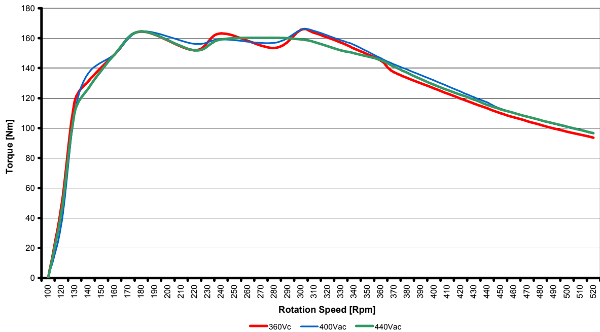
Torque Curve
